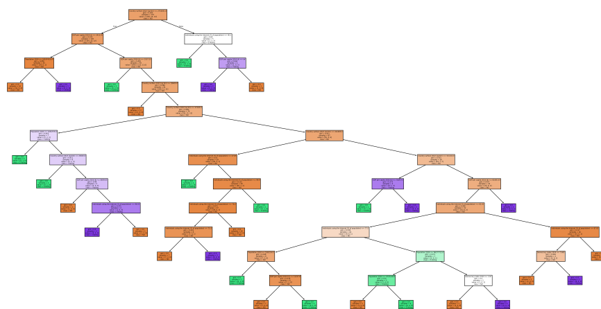
Figure 7. The three-class decision tree.
