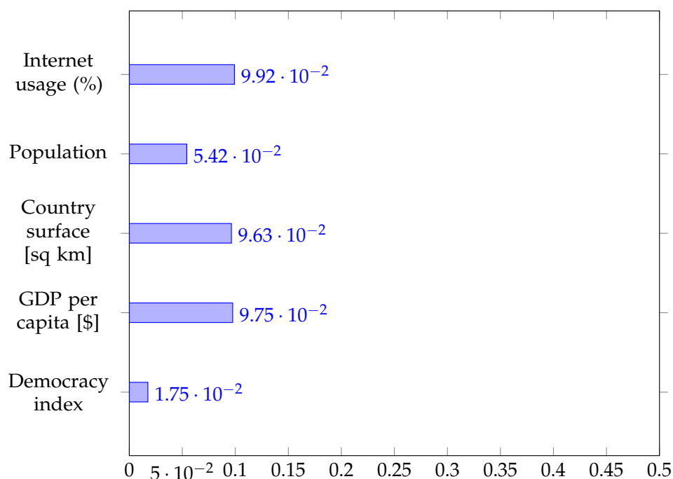
Figure 10. Mean decrease of Gini impurity index for three-class decision tree.
