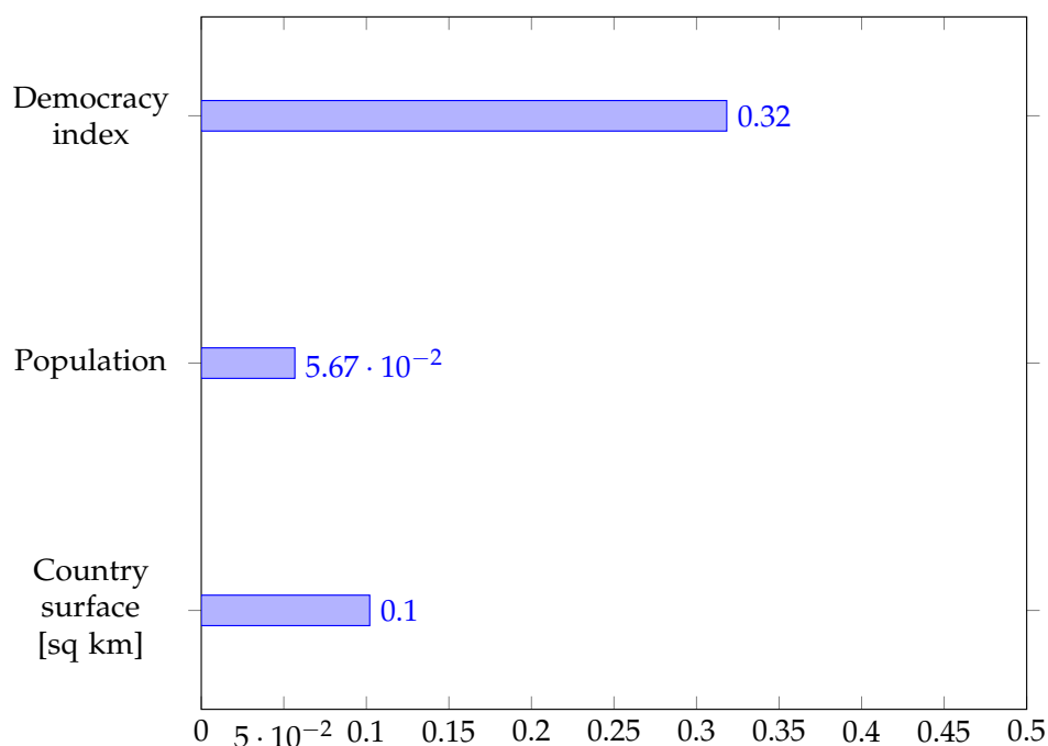
Figure 12. Mean decrease of Gini impurity index for the second stage of the cascade of two-class decision trees (e-voting vs i-voting).
